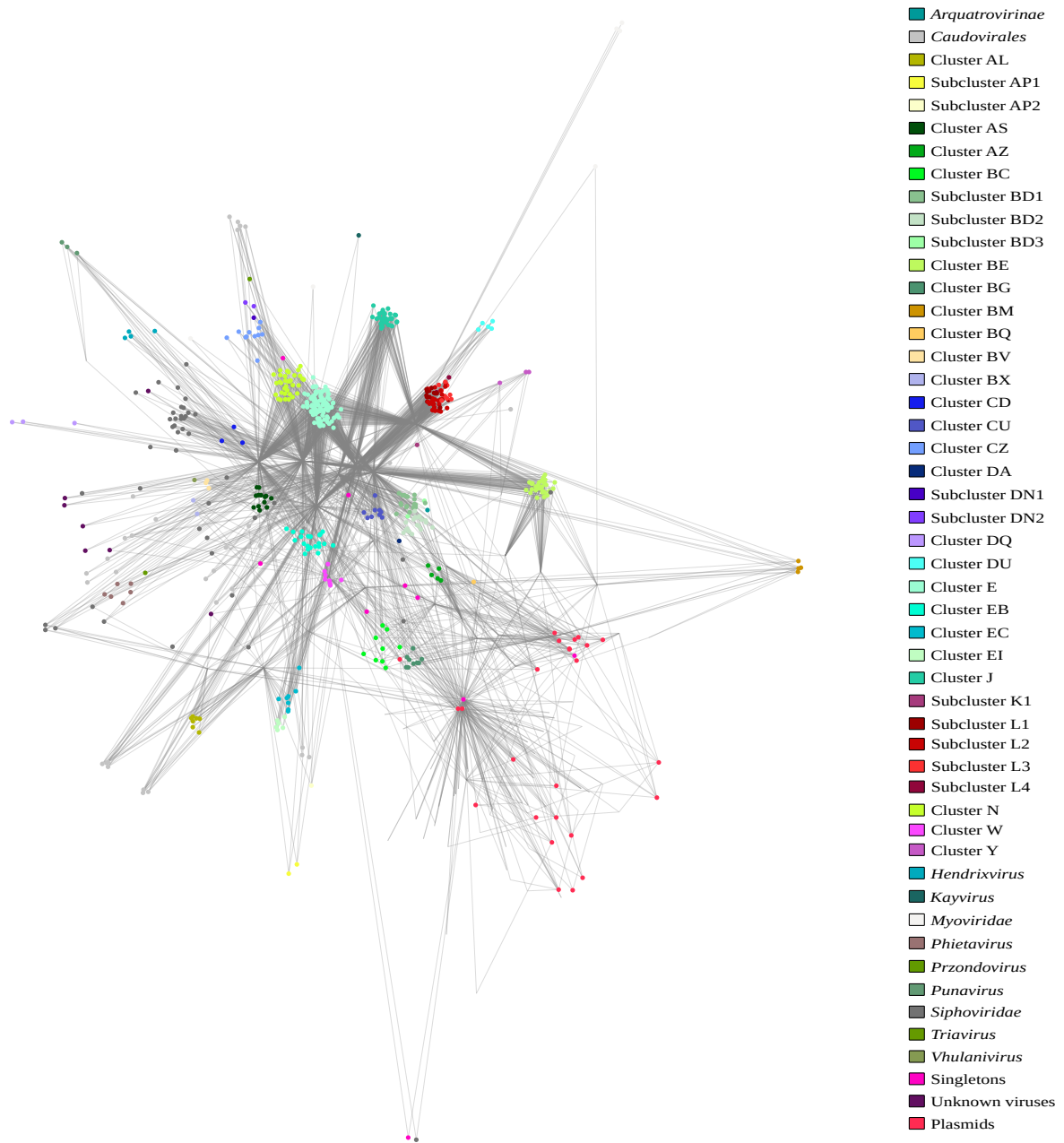
Fig. S6. Bipartite network reflecting genome nodes and edges of Streptomyces phage Gilgamesh, phages and plasmids containing homologs of Gilgamesh proteins. Genome nodes are marked with colored circles, cluster nodes are not marked. The edges reflect the homologous clusters with Gilgamesh proteins. The node of Streptomyces phage Gilgamesh is marked with red ellipse.
